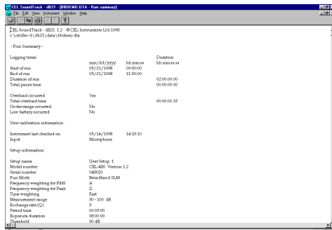
summary screen showing run information
